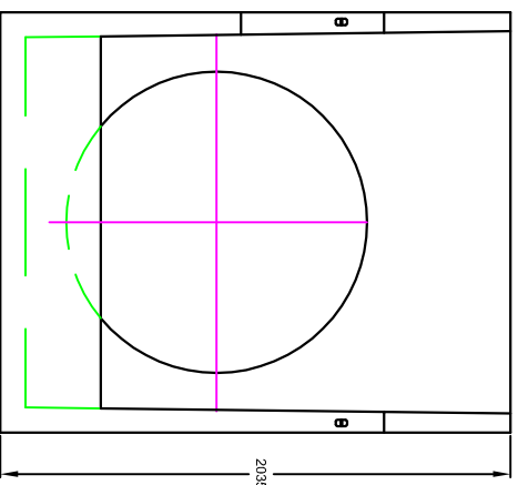
Front elevation with grating removed.
